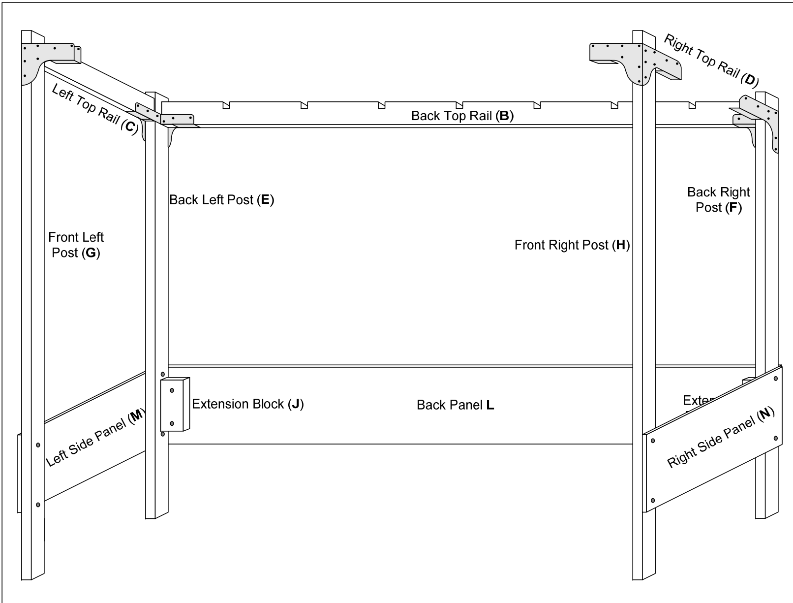
Figure #8: Attach Front Right Post (H) to the Right Side Panel (N)
