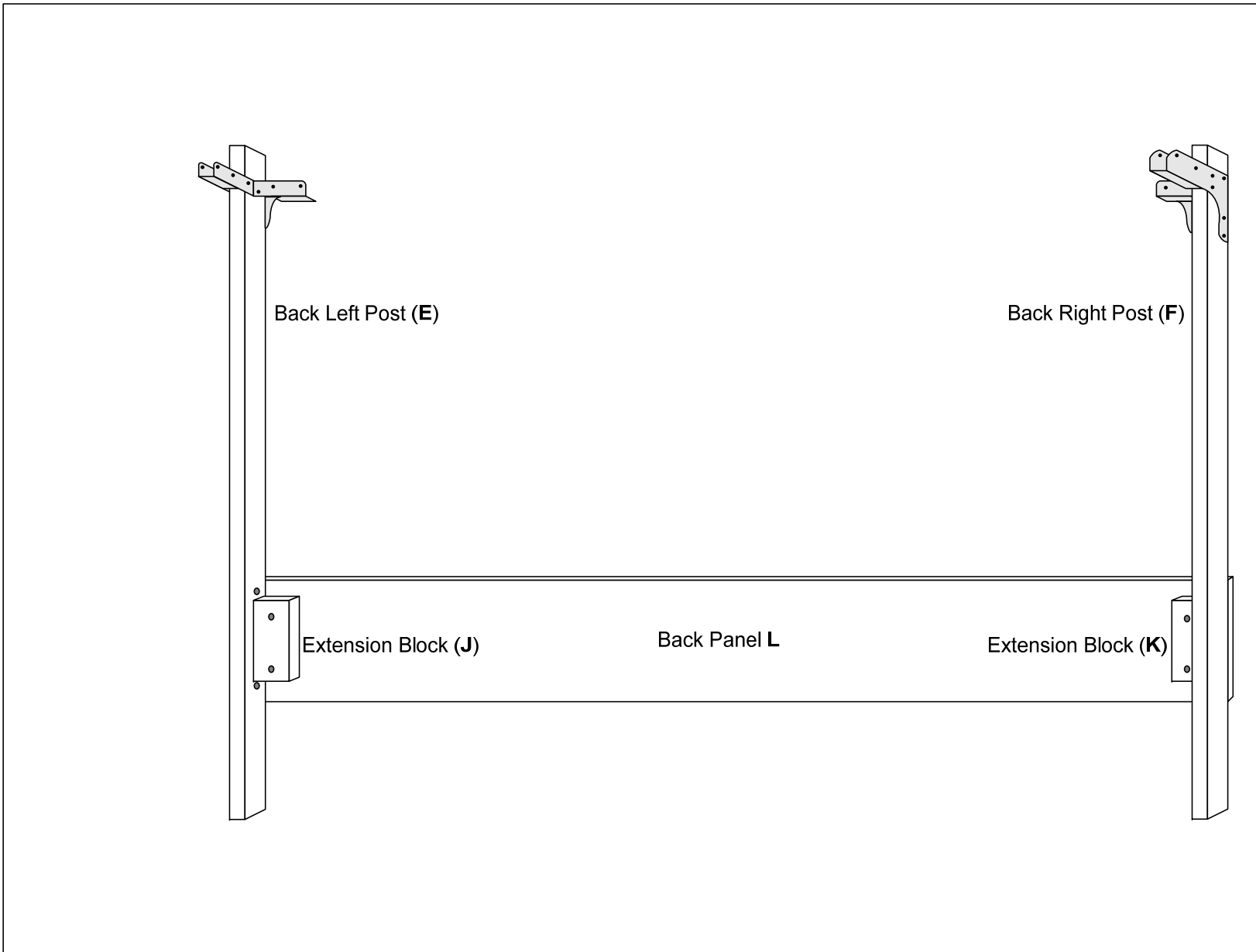
Figure #2: Attach Back Panel (L) to Extension Block (K) on the Back Right Post (F)
