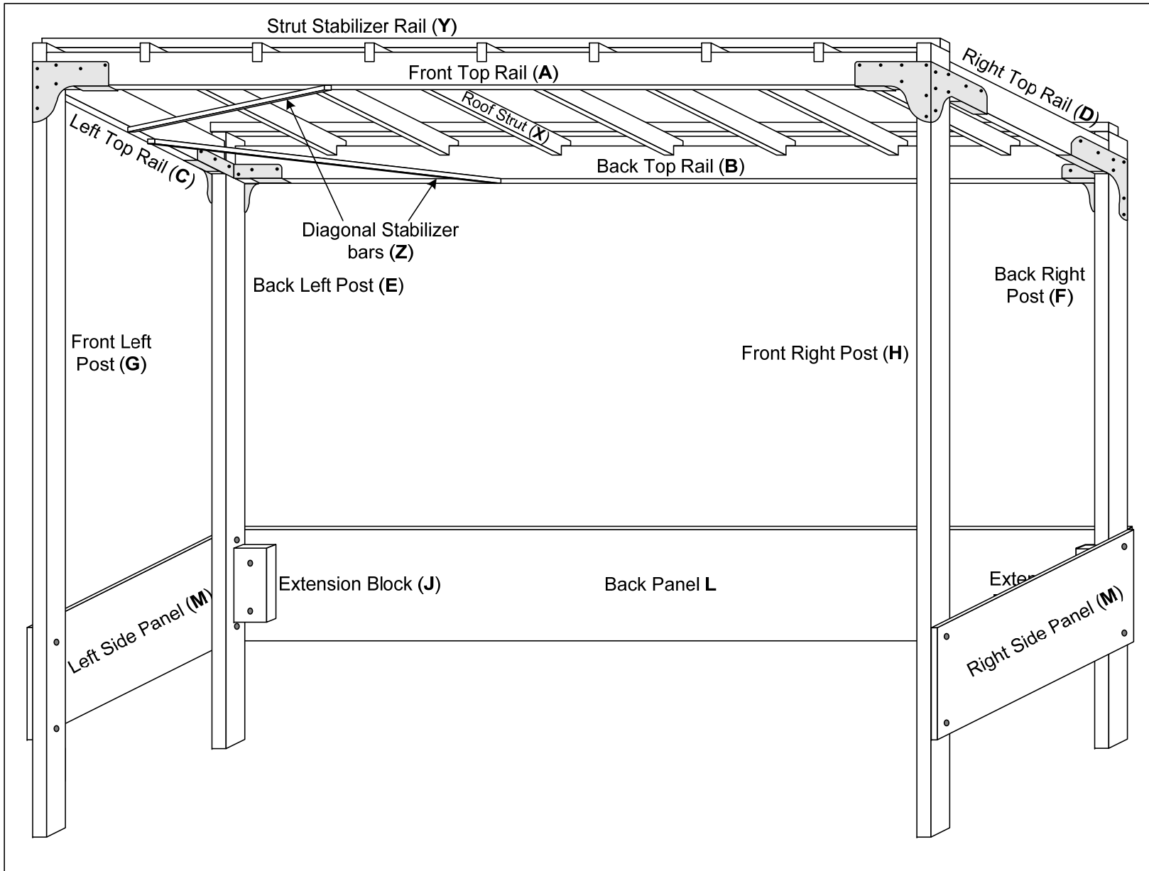
Figure #13: Attach Diagonal Stabilizer Bars (Z) to Left Top Rail (C) and to Front Top Rail (A) and Back Top Rail (B)
