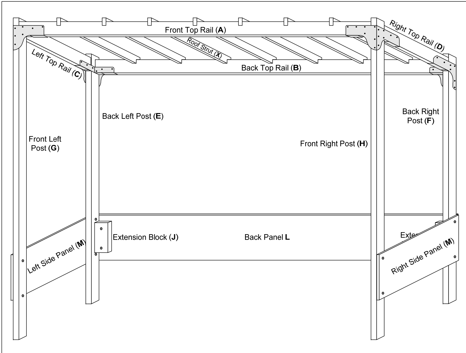
Figure #11: Insert Roof Struts (X) into slots in Front Top Rail (A) and Back Top Rail (B)
