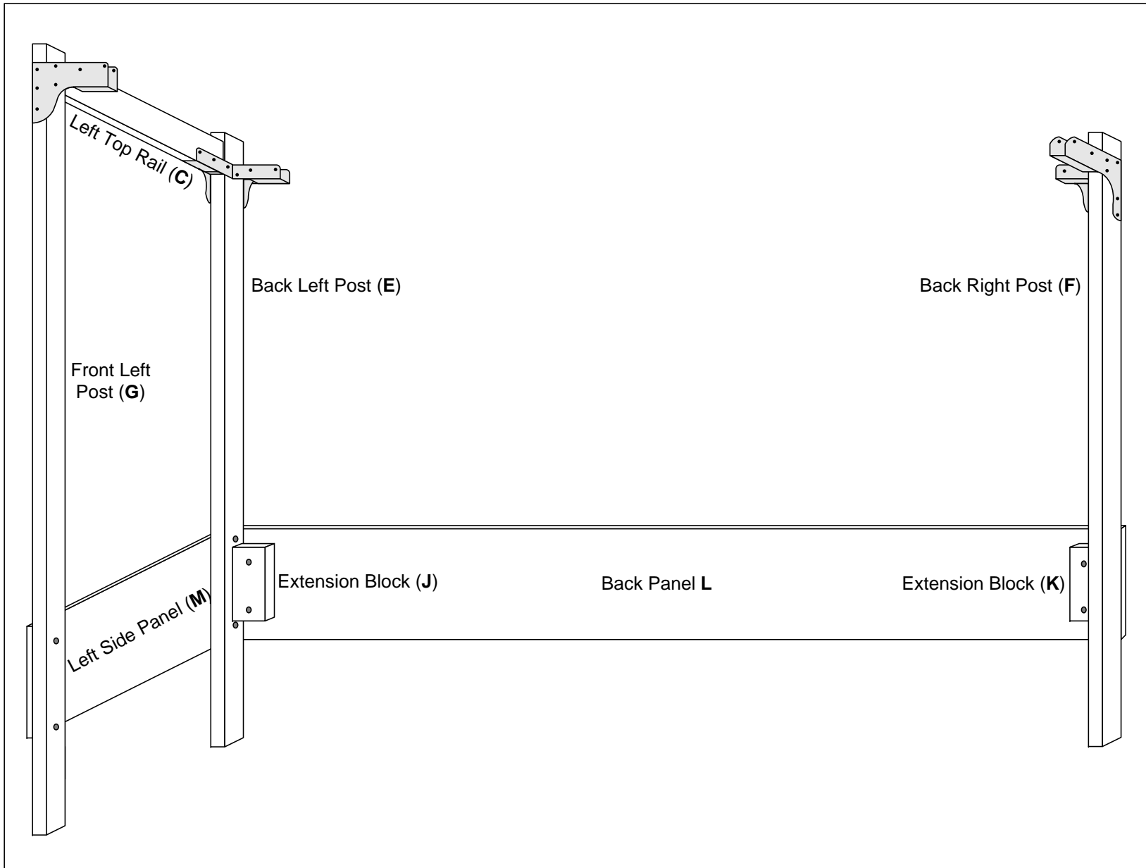
Figure #5: Insert Left Top Rail (C) into the brackets on the Back Left Post (E) and Front Left Post (G)
