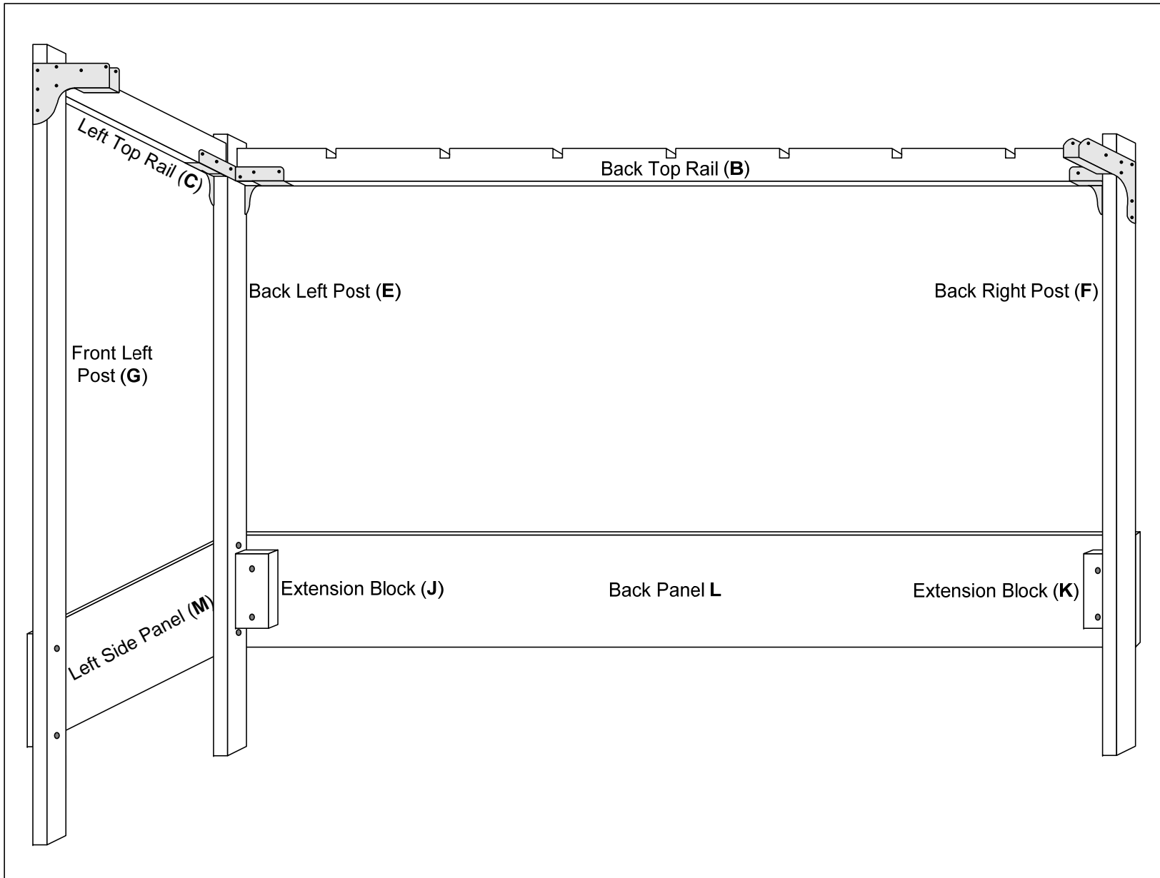
Figure #6: Insert Back Top Rail (B) into the brackets on the Back Left Post (E) and Back Right Post (F)
