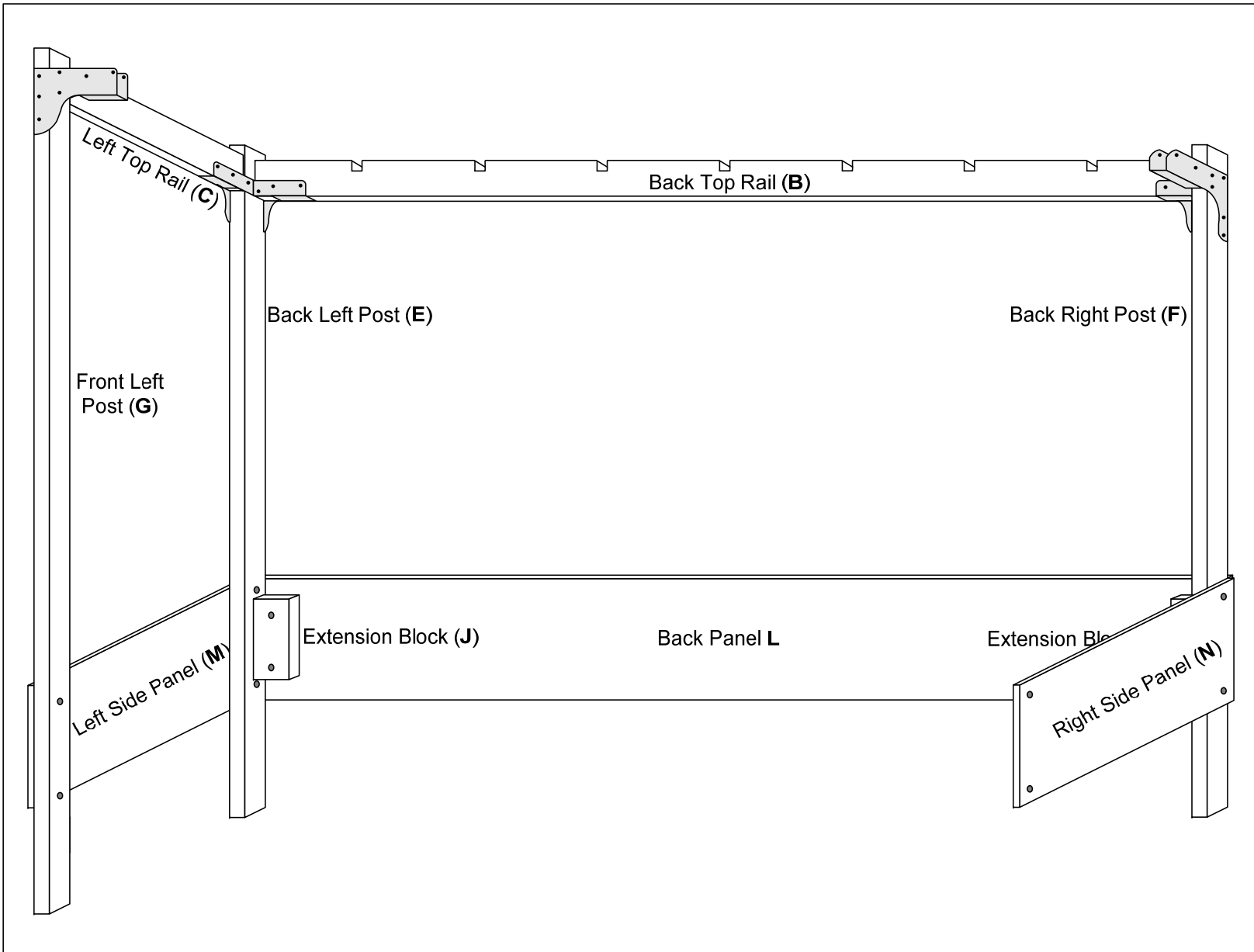
Figure #7: Attach Right Side Panel (N) to the Back Right Post (F)
