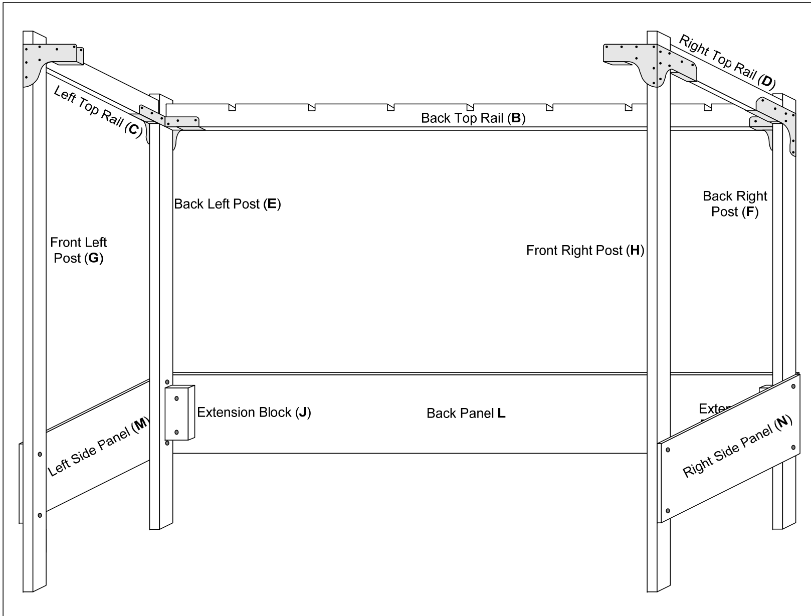
Figure #9: Insert Right Top Rail (D) into the brackets on the Back Right Post (F) and Front Right Post (H)
