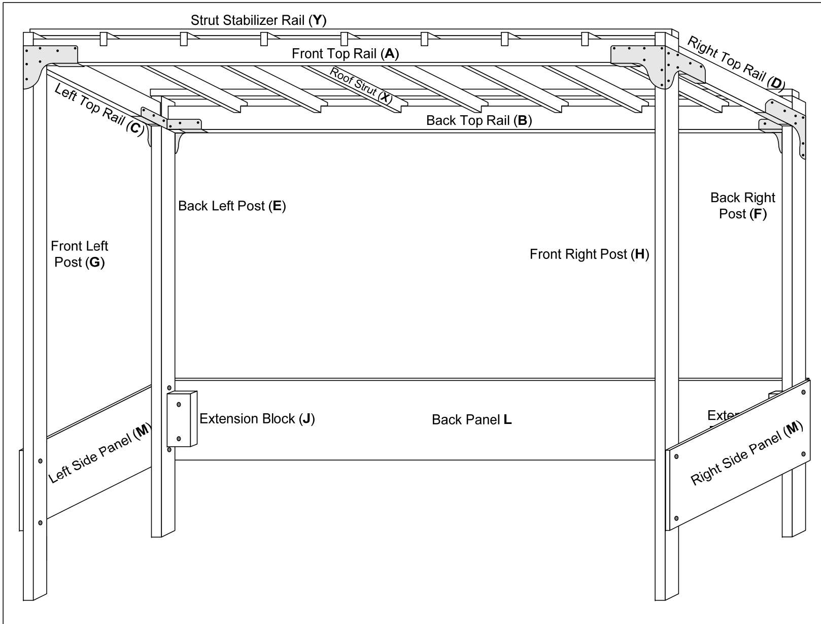
Figure #12: Attach Front and Back Roof Strut Stabilizers (Y) to hanger bolts in top of Corner Posts
