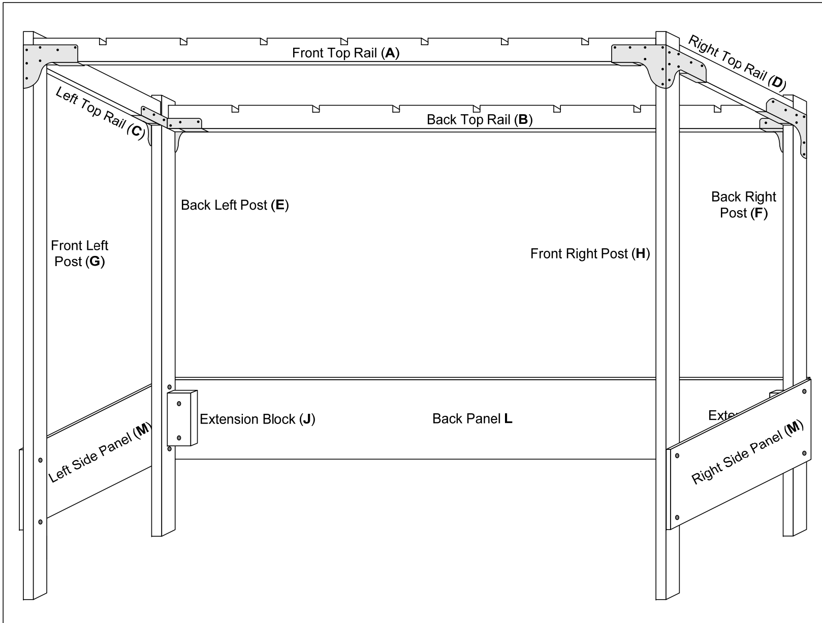
Figure #10: Insert Front Top Rail (A) into the brackets on the Front Left Post (G) and Front Right Post (H)
