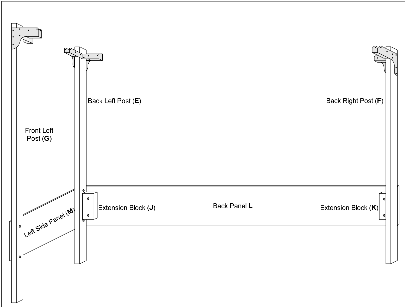
Figure #4: Attach Front Left Post (G) to the Left Side Panel (M)
